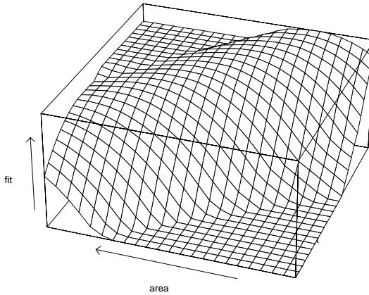
Figure 8.10: A two-dimensional fitted section of a projection pursuit regression surface fitted to the rock data. Note that the prediction extends the ridge functions as constant beyond the fitted functions, hence the planar regions shown. For display on paper we set drape = F .
