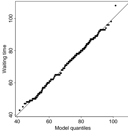
Figure 16.2: Sorted waiting times against normal mixture model quantiles for the ‘Old Faithful’ eruptions data.
